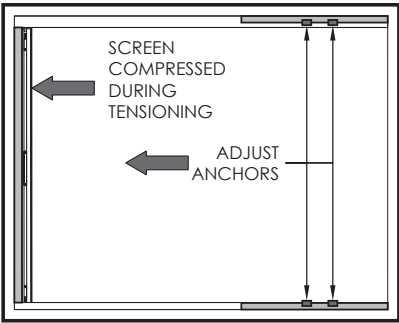
4. Tension cords
